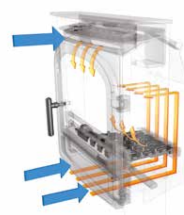
INSET AIRFLOW
